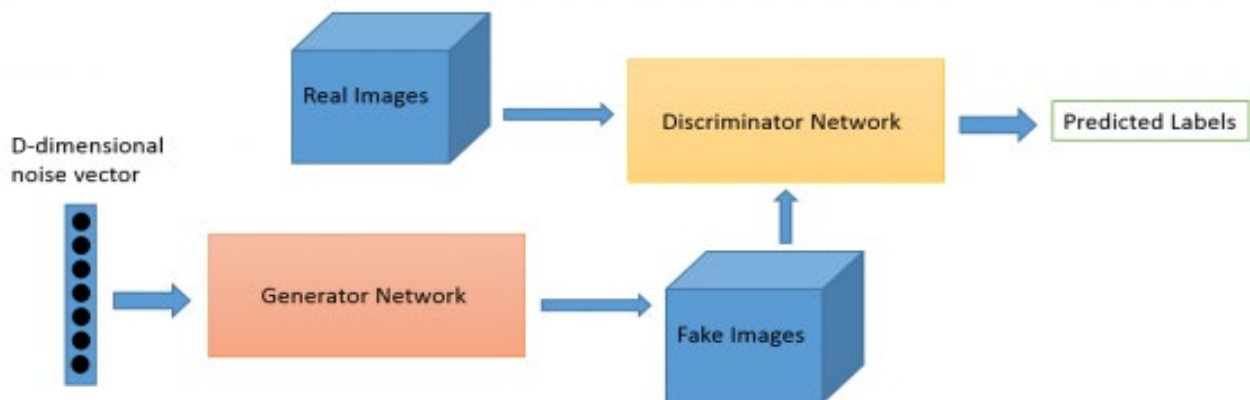
Figure 1 – Example of GAN
