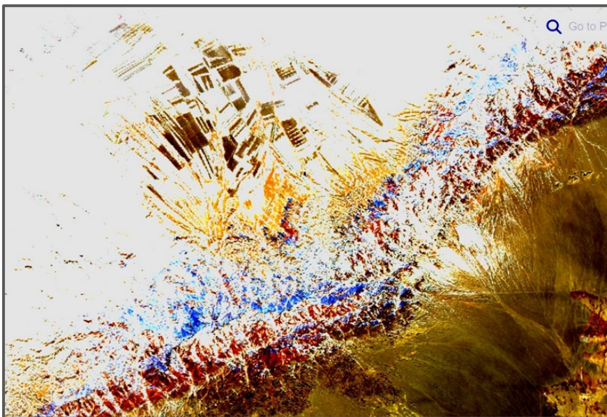
Fig. 5. Melting of snow on the spurs of the Dzungarian ridge and agricultural fields in winter (01.16.2025) due to the heat flow from the Ili Valley (Sentinel-2).
