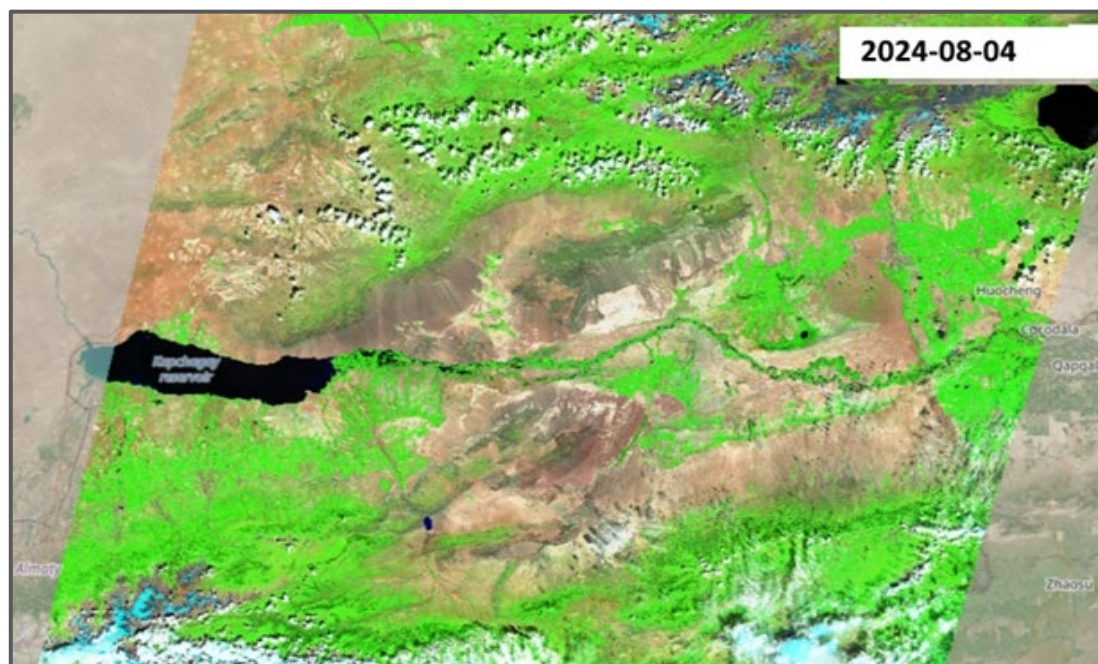
Fig. 3. The Ili River Valley as seen from Sentinel-2, August 4, 2024.
