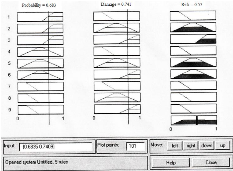
Figure 1.6 The inference engine (on the output values)
