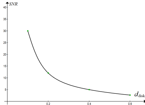
Fig. 4. Dependence of SNR on pinhole size
