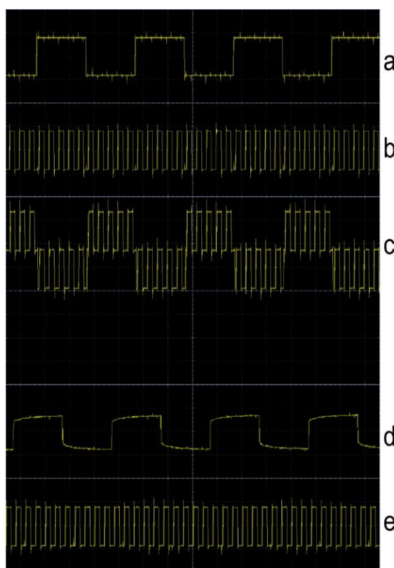
Fig. 3. Result of demultiplexing information signals
