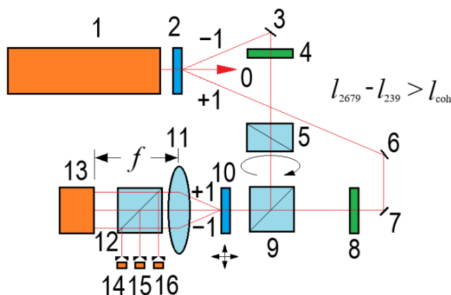
Fig. 2. Experimental setup for testing the performance of singular multiplexing
